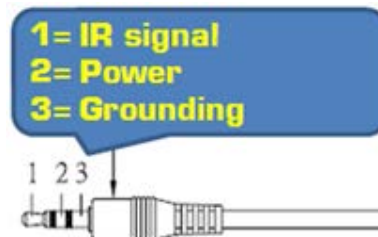
IR Receiver
